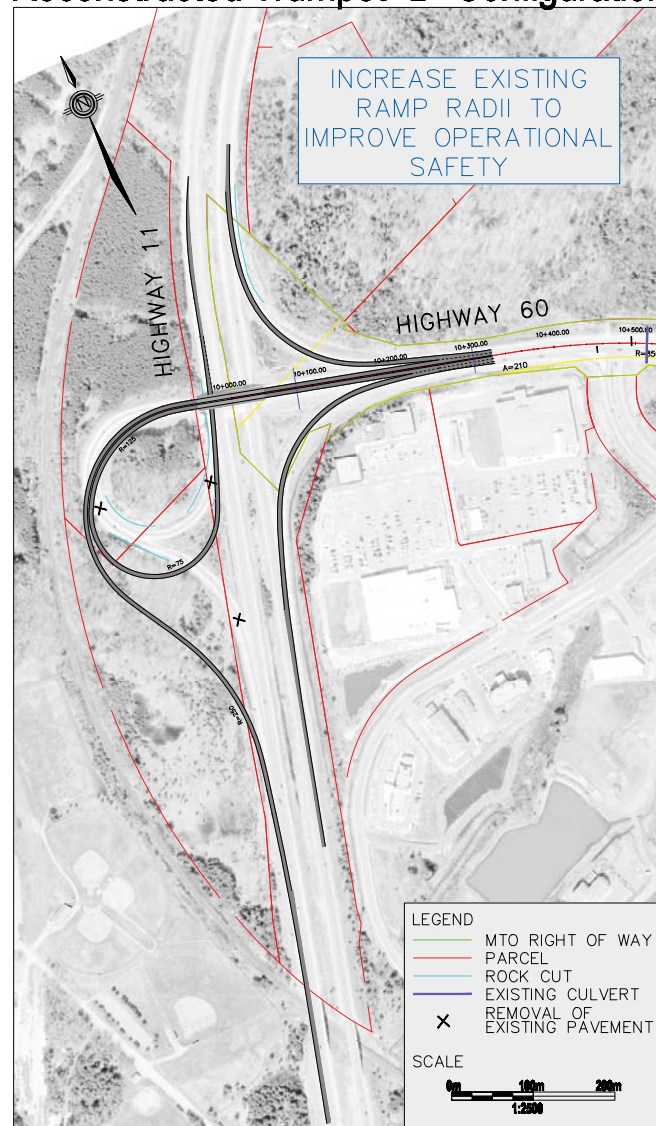
Alternative 1A-2: Reconstructed Trumpet "B" Configuration
