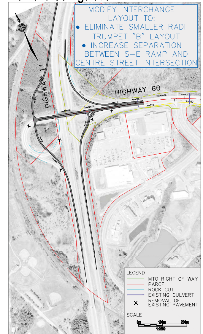
Alternative 1A-5: Diamond Configuration
